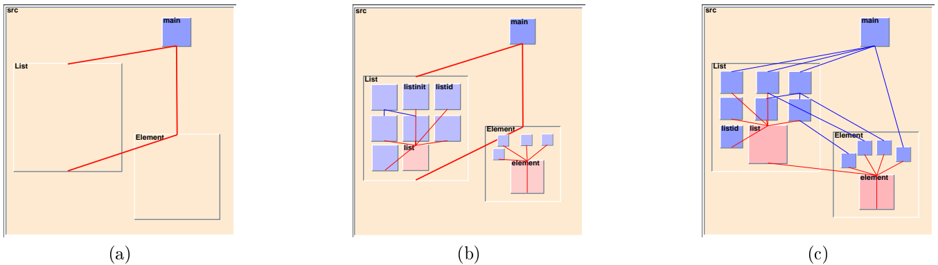
Figure 3: (a) This window presents a main function and two subsystems List and Element as before. (b) The List and Element nodes have been opened to display their children and show an overview of the hierarchy. (c) Composite arcs have been opened to display the constituent lower-level dependencies.
